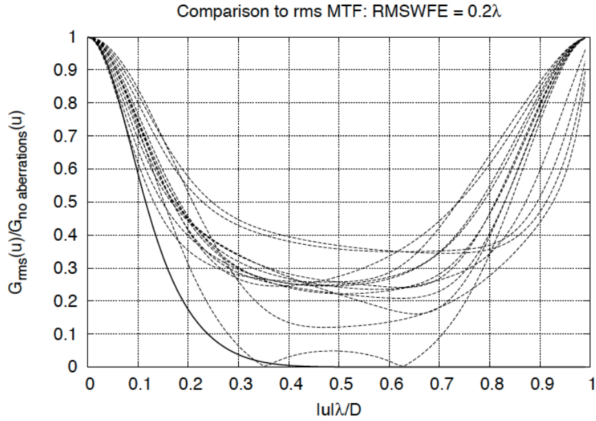
Figure 2: The rms MTF for an unobstructed aperture with aberrations, relative to the unaberrated case at \text{RMSWFE} = 0.2\lambda . The solid curve is the fitting formula used in the ETC. The dashed curves are low-order aberrations. There are 13 cases shown, with different aberrations: defocus, astigmatism, coma, and trefoil; and cases with 25:75, 50:50, and 75:25 mixtures of defocus with the other three aberrations.
